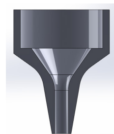
5mm nozzle
